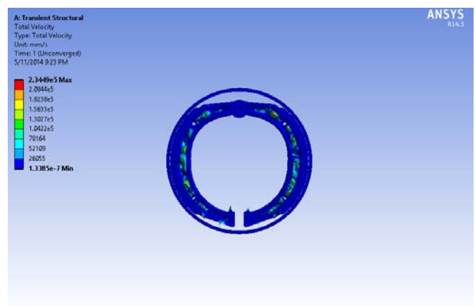
Figure.20 – 80 kmph speed
