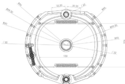
Figure.9 Front brake assembled front view with dimensions
