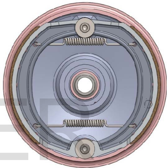
Figure.6 Front brake assembled front view
