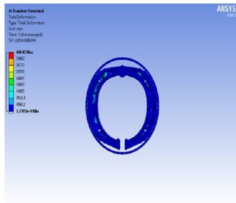
Figure.15 – 60 kmph speed
