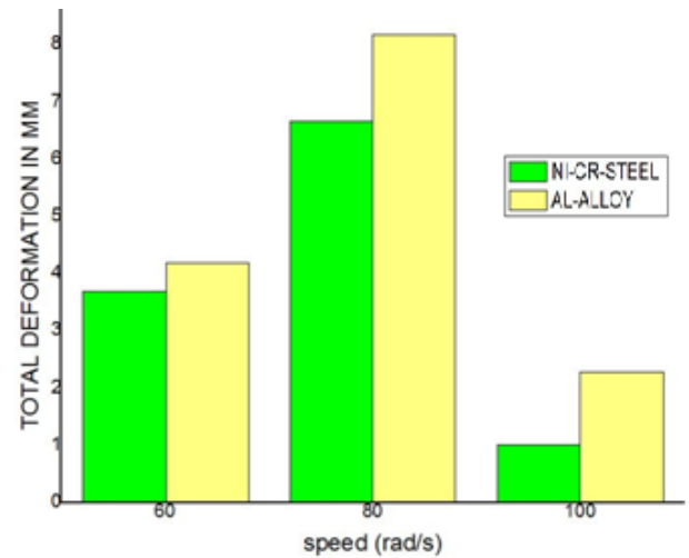
Figure.18 Total deformations at different speeds
