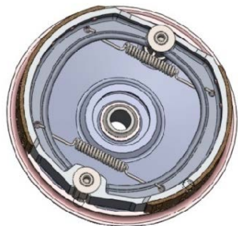
Figure.7 Front brake assembled isometric view
