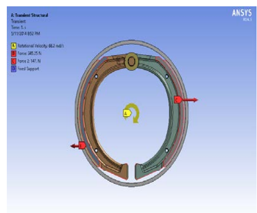
Figure.14 Applying Loads and supports
