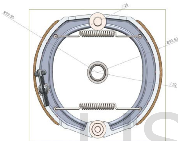
Figure.9 Front brake assembled front view with dimensions
