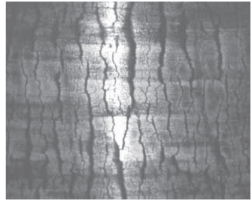
Figure.1 Brake rotor surface showing a high level of heat checking.
