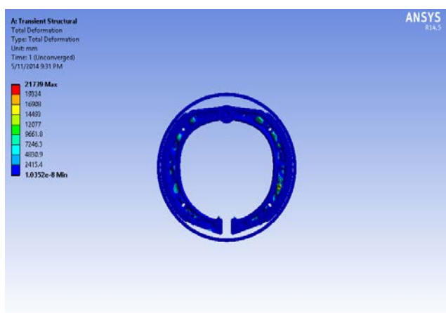
Figure.17 –100 kmph speed
