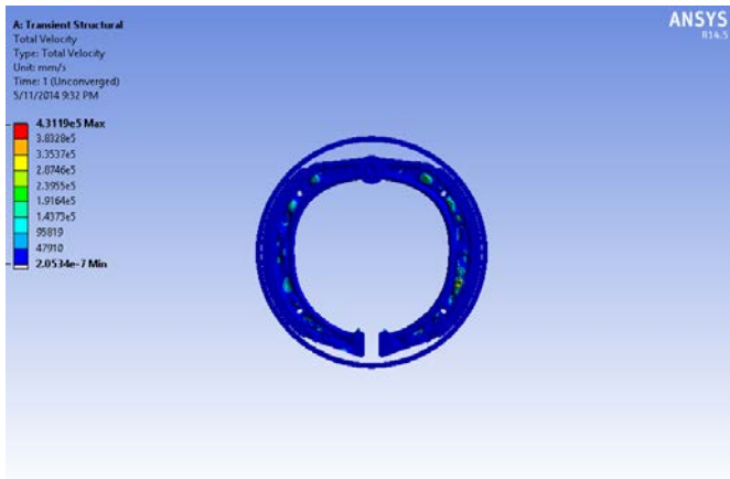
Figure.21 – 100 kmph speed
